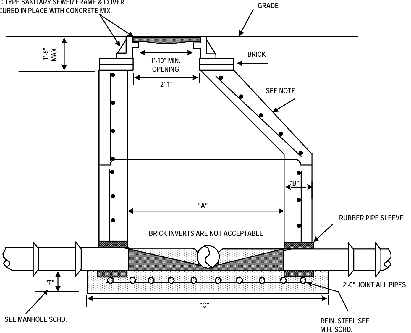
TYPICAL MANHOLE DIMENSIONS
